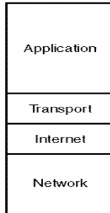
TCP/IP MODEL
