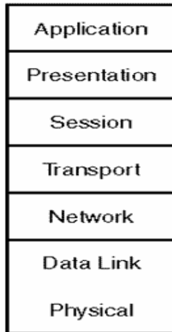
OSI MODEL
